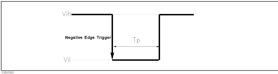
Figure 7-2. RUN/CONT Trigger Signal
